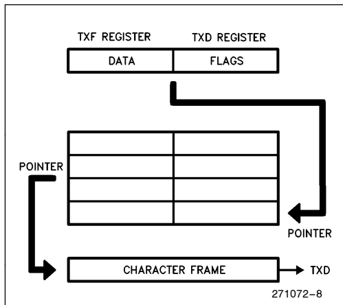
Figure 8. Tx FIFO
